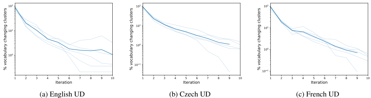
Figure 2: Number of words that participate in swaps as the iterations progress. Individual runs are shown in pale blue, and the mean in a stronger tone.
