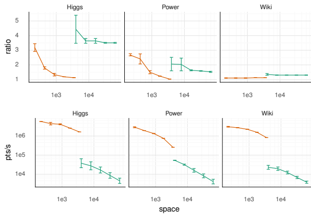
Figure 4: Approximation ratio (top) and throughput (bottom) versus space for CoresetOutliers (in orange) and BaseOutliers (in green). CoresetOutliers uses space \mu(k+z) , with \mu = 1, 2, 4, 8, 16 , BaseOutliers requires space m(k \cdot z) , with m = 1, 2, 4, 8, 16 ( \mu and m increase from left to right in each plot). Space and throughput are in logarithmic scale.
