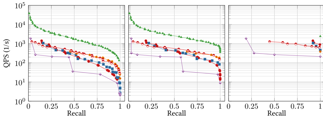
Figure 8 (Approximate) Recall-QPS (1/s) tradeoff - up and to the right is better, GIST dataset, 100-NN; left: \epsilon = 0 , middle: \epsilon = 0.01 , right: \epsilon = 0.1 .
