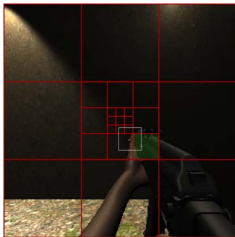
Figure 2: The VPR is more fine grained in the direction the gun is pointing. Shown is an example of the DCNN correctly predicting the class (green square) with a confidence of 55.7%, with only four pixels of the target being visible.
